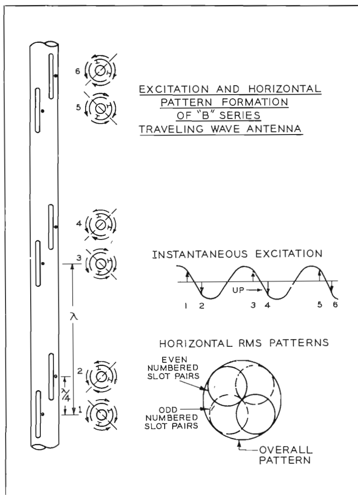
FIG. 8. This is the main aperture arrangement for a B-series Traveling Wave Antenna. Note the differences between the A-series as shown in Fig. 3, the resulting pattern is the same.
