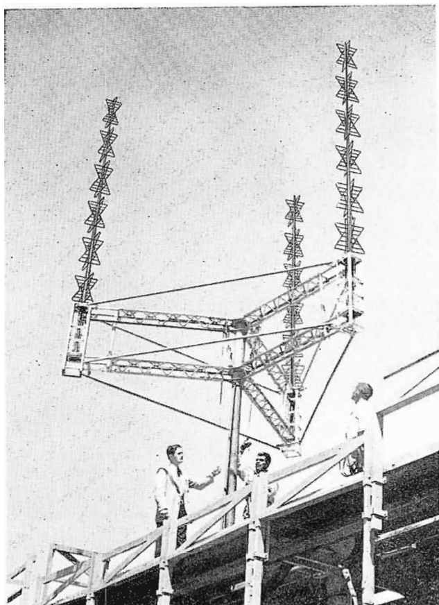
FIG. 3. Extensive testing proved the feasibility of this Candelabra system. A scale model, shown here, was constructed by RCA to determine the exact spacing of the antennas and their effects upon each other. The accuracy of this small model has been proved in the performance of the completed structure.
