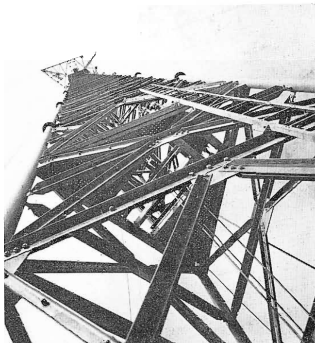
FIG. 4. The solid steel legs of the tower are shown here. Extra strength is obtained from the elaborate cross bracing in the tower. Note that when this photograph was taken the erection was in progress.
