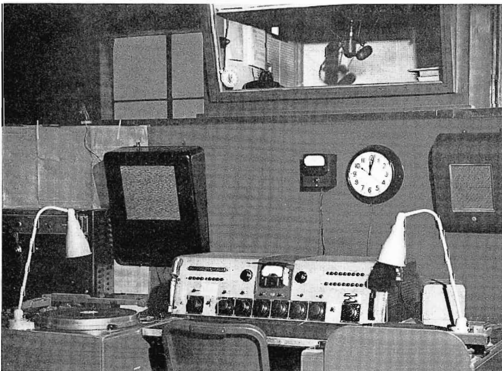
FIG. 12. WTOP originates its all-night show from this small announce booth at the transmitter site. The series 76 consolette and two turntables are all the studio equipment needed. Normal sound isolation, used in the booth, is sufficient to make room noise from the transmitters inaudible.
