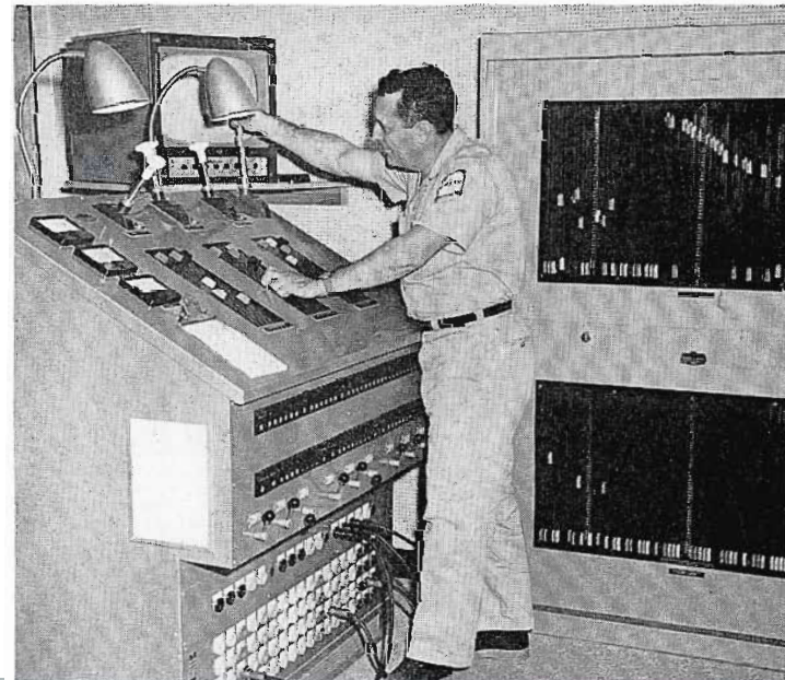
FIG. 11. Tony Maggiore, supervisor of camera and lighting is shown operating the Aerial-Davis lighting board located in production control. Panel to right is Quick Connect Board which can handle 120 20-amp. circuits with no patch cords. Sloping panel to left has 21 dimming circuits. Circuit breakers and transfer switches are directly below dimmers and 72 50-amp. patch circuits are here at knee height. Total capacity of equipment is 200 kw.
