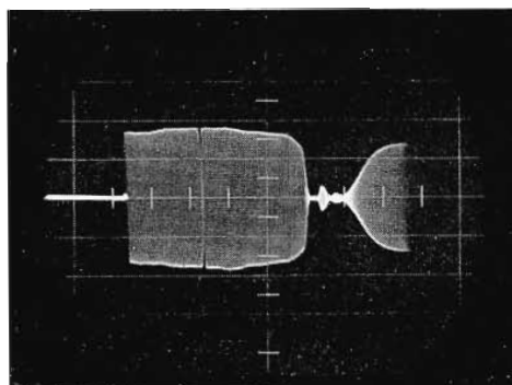
(A) Same as 8(A) but for dual channel sound. Note three notches in response, at 6.2 mc, 6.8 mc, 7.16 mc (7.16 mc notch).
