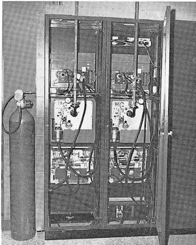
FIG. 19. Rear view, microwave receivers at transmitter.
