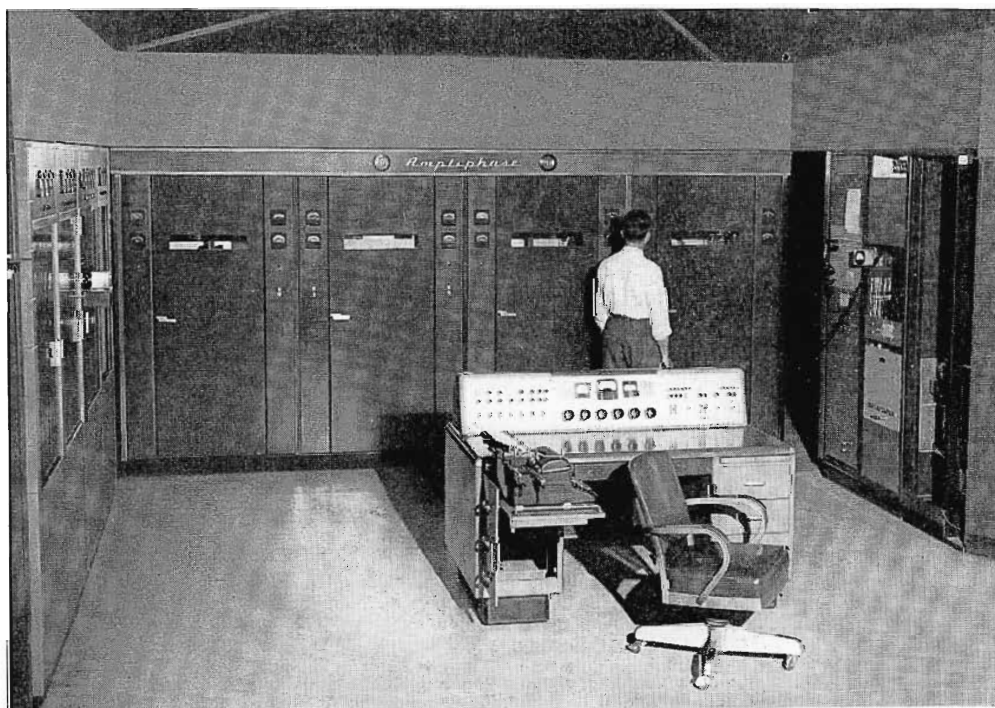
FIG. 2. All operating equipment is concentrated in the center of the circular transmitter room. The 10-KW BTA-10H Transmitter can be seen on the left, and the Ampliphase 50-KW Transmitter cubicles are in the center. Phasing and input equipment is on the right.
