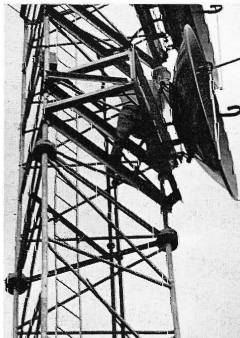
FIG. 22. Engineer lining up microwave dish by means of sighting tube placed on top of it.
