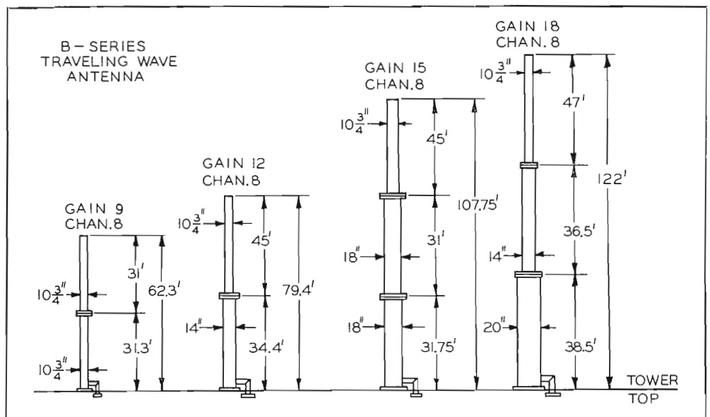
FIG. 12. Major dimensions of the B-series antennas are shown here.
