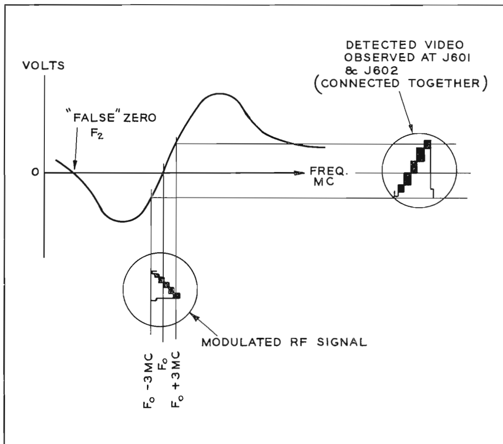
FIG. 3. Sketch illustrates correct adjustment of discriminator cavity for detecting frequency modulated signal and supplying error voltage to AFC.
