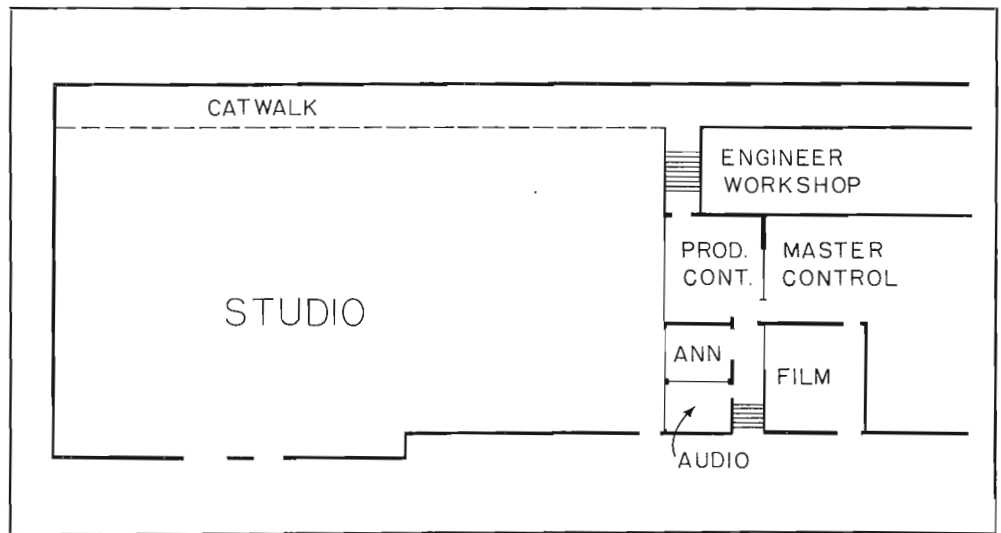
FIG. 10. First floor plan of WWL-TV studio building, showing how the technical facilities are arranged. Note that Production Control and Master Control are separated. This gives the technical personnel an area of their own in which to operate, without distraction. Likewise, the director, agency, and client can have privacy in their own area. Also, video and audio engineers are separated. The Announcer is located between Production Control and Audio. The Film room is directly behind Audio and Announcer. Under this arrangement, all can see into the other's area, and all can see into the studio.
