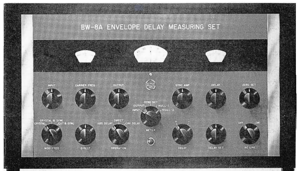
FIG. 4. This is the Type BW-8A Envelope Delay Measuring Set. All control functions are on the front panel for ease of operation.
