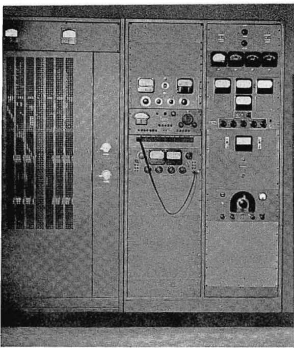
FIG. 10. This shows a portion of the phasing equipment (left) and the monitoring equipment located in the two standard size racks.
