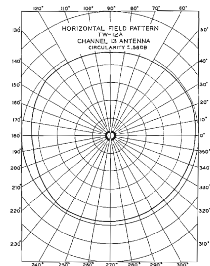
FIG. 5. The measured horizontal field pattern of a TW-12A (gain of 12) Channel 13, shown here, is for a typical A-series antenna.
