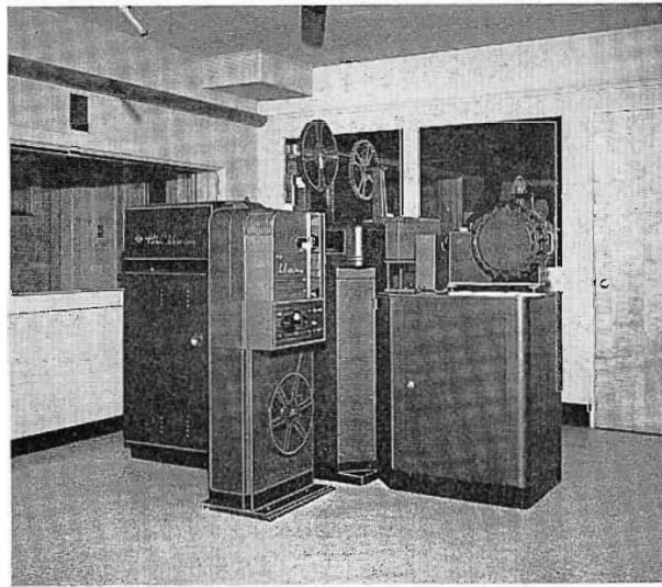
FIG. 7. Projection room with two TP-6CC Film Projectors, a TP-7 Slide Projector, a TP-15 Multiplexer, a 1-V Vidicon Film Camera and a 3-VColor Film Camera. Space left for a duplicate of this set-up is now in process of having equipment installed. (Access holes in floor for this expansion were plugged at the time that this picture was taken).
