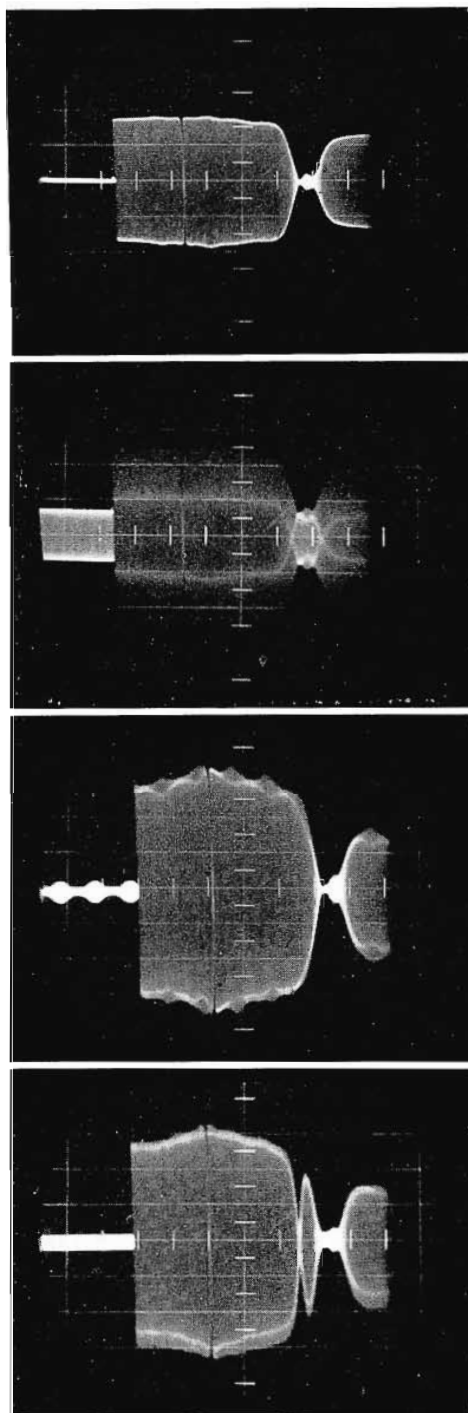
FIG. 8. Waveforms of single channel sound diplexer filter responses and alignment signals.
