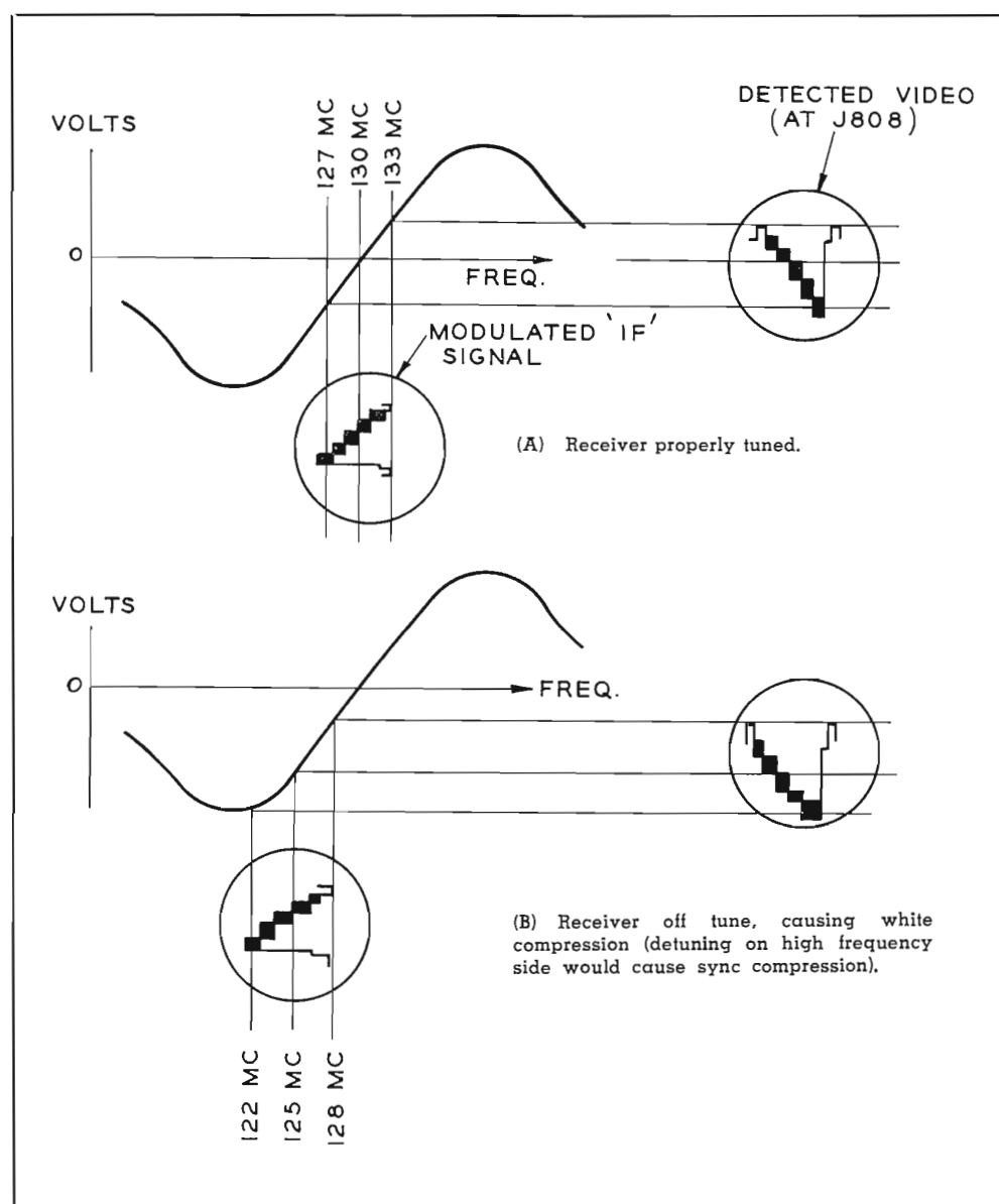
FIG. 4. Receiver IF discriminator characteristic is adjusted at factory. Whether it is utilized at center (130 mc) depends on receiver local oscillator setting, and ability of AFC to hold on zero error voltage.
