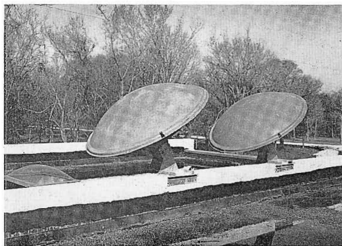
FIG. 17. Front view of microwave dishes mounted on roof of transmitter building. (Note protective plastic covers on dishes).
