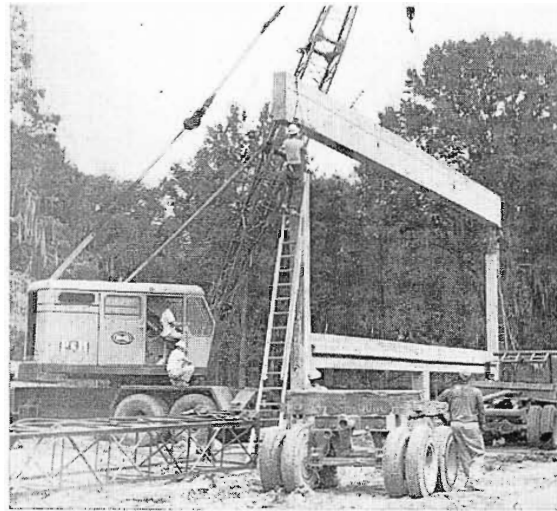
FIG. 26. Installing the first of four 14-ton prestressed concrete beams, which allowed an unobstructed floor area of 50 by 60 ft. In spite of inclement weather the prestressed concrete building was assembled in three days.
