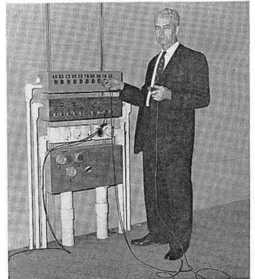
FIG. 3. Francis Jacob, Jr., chief engineer of audio facilities, at one of four termination panels in studio. Each contains 10 microphone, 9 audio and 2 video outlets; 2 intercom system, and 3 camera outlets. Conduit is in place for 3 more camera cables for color cameras.
