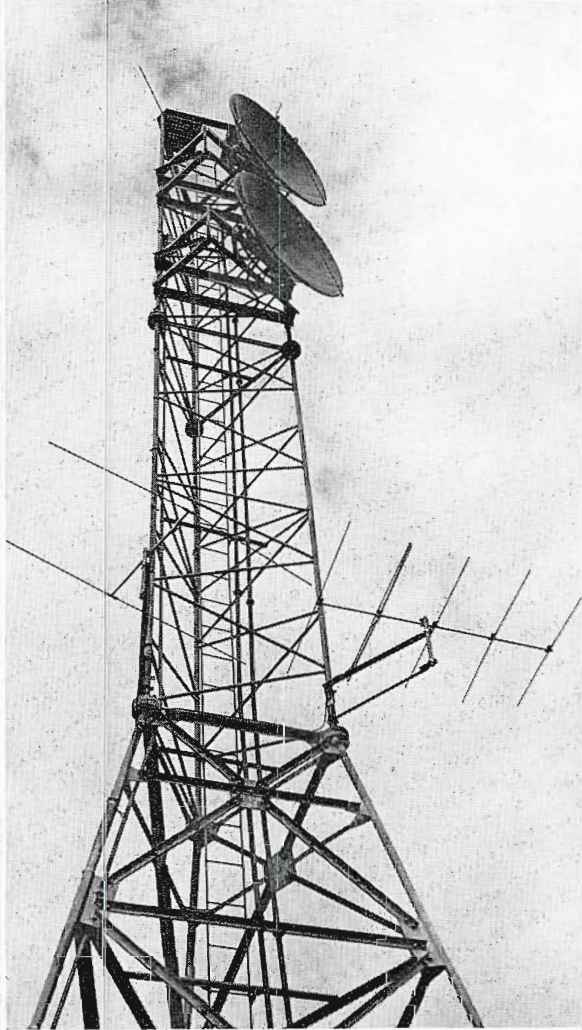
FIG. 15. Tower atop studio building shows mounts for microwave dishes, (also receiving antennas for office monitoring system). This tower is 67 feet high, (90 feet above street or sea level).
