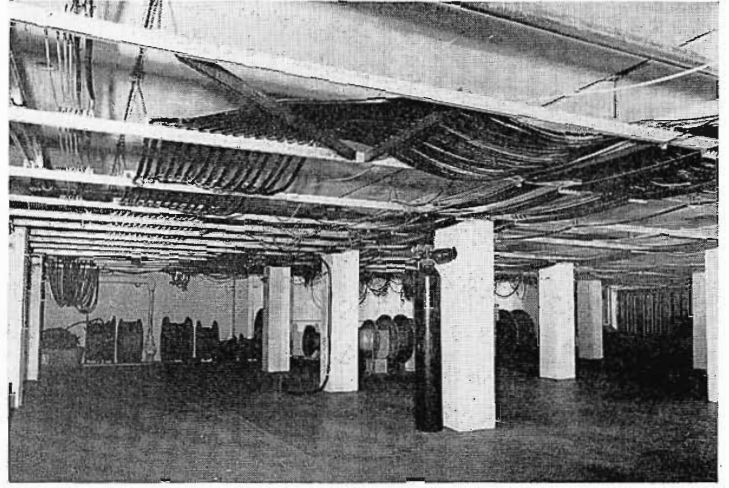
FIG. 6. The wiring vault beneath master control. Utilizing the 5-foot elevation of master control room, the suspension of a power-strut grid permits easy addition or removal of cables and video lines, without disturbing existing wiring. Note the absence of cable trays or raceways. Ten-inch holes under each piece of equipment provides cable access and permits exhausting of filtered, cool studio air through equipment racks.
