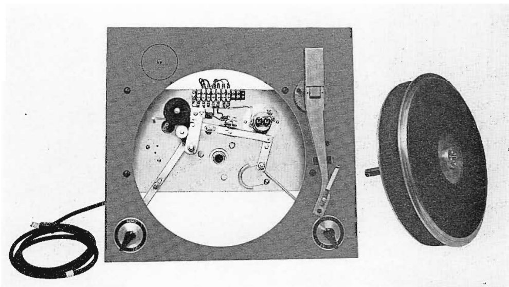
FIG. 3. The platter assembly is easily removed exposing the idler wheels and wiring terminals. Lubrication is thus simplified.
