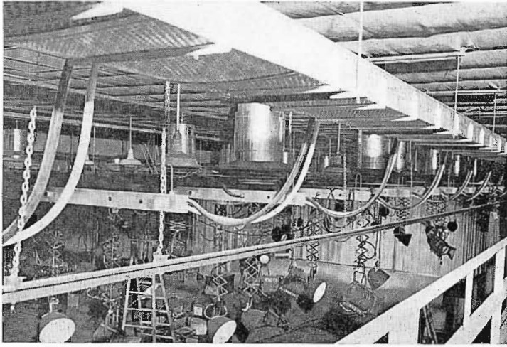
FIG. 5. View of light battens hung by chain from power-strut channel. Battens, which average 25-ft. in length, contain 6 20-amp. receptacles and 4 50-amp. receptacles with channel for hanging fixtures. The fiberglass acoustical treatment, as seen in this photo, is covered by fiberglass screen. Note flexible cables to permit batten movement.
