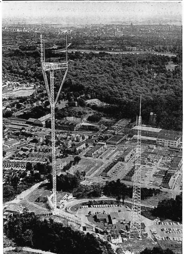
FIG. 2. The Candelabra System overlooks the entire city of Baltimore. Here the new structure is shown in comparison to WJZ's old tower. The suburbs of Washington, D. C. can be seen from the platform on a clear day.
