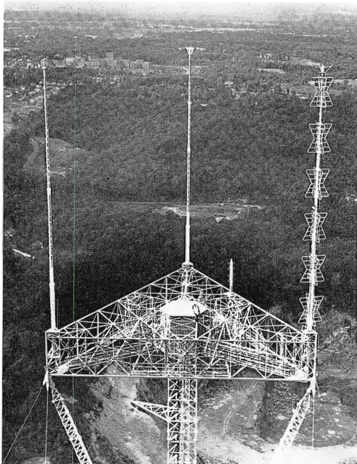
FIG. 9. The platform, shown from the air, begins at the 625-foot level. The two Traveling Wave and one Superturnstile antennas are mounted on the corners of the platform. In the center is the penthouse, connecting with each antenna by catwalks. One of the microwave dishes and a standby two-bay superturnstile antenna can also be seen.
