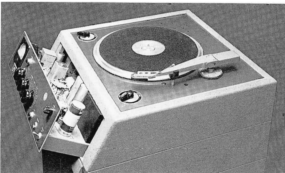
FIG. 4. This shows how the BA-51A Magnetic Record/Reproduce Amplifier is installed in the turntable cabinet and it is easily removed for servicing.
