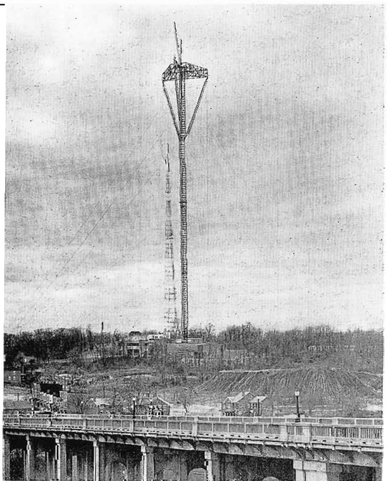
FIG. 15. The Candelabra is shown in contrast to the surrounding terrain. The overall height of the structure is approximately 1000 feet above sea level; however, the physical height of the structure is 730 feet.
