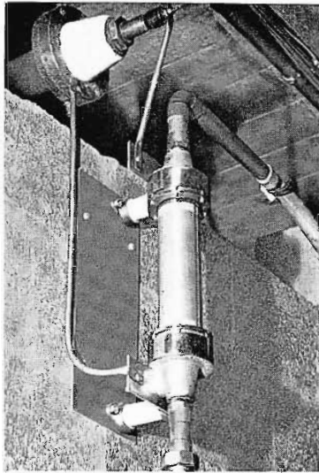
FIG. 11. The wire wound 50-kw dummy load is mounted in the basement just below the transmitters. This unit is capable of dissipating full power generated by the 50-KW Ampliphase Transmitter at 100 percent modulation. A flow of only 15 gallons per minute of ordinary tap water are required for complete cooling of the load.
