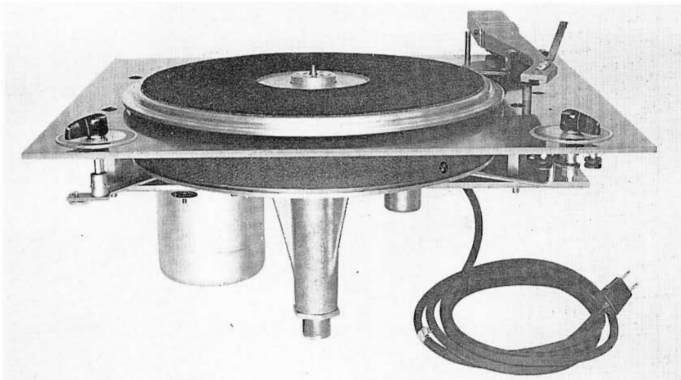
FIG. 2. The BQ-51 easily mounts in custom installations. The mechanism shown here can be mounted with no other components required.
