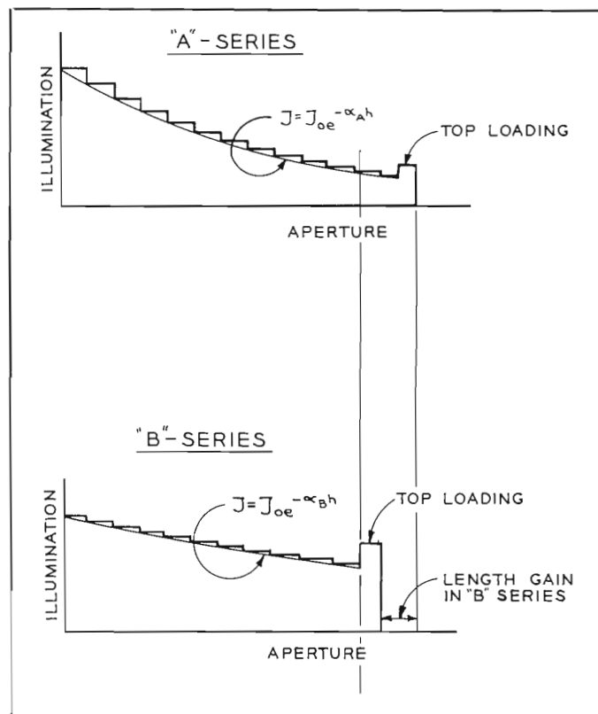
FIG. 9. Note the differences in the distribution of the illumination of "A" and "B" Series Antenna for the same gain. The illumination of the B-series is more uniform because of the lower attenuation rate and the higher top loading energy. Shorter overall length of B-series as a result of the higher aperture efficiency, is also illustrated.
