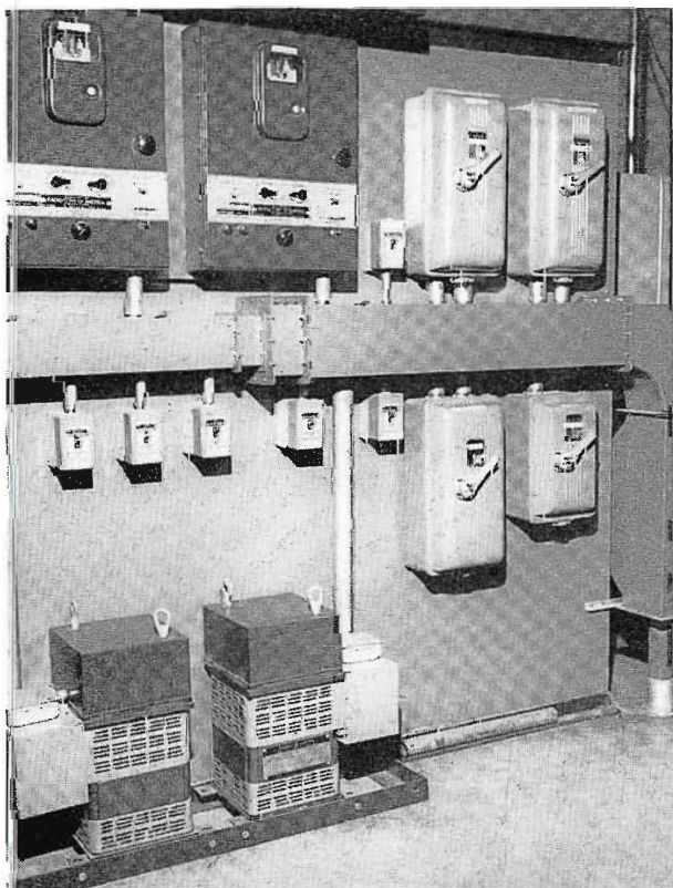
FIG. 8. Switchgear for the Ampliphase Transmitter has been mounted on this \frac{3}{4} -inch plywood panel with angle iron frame. This arrangement provides easy access to all components. Voltage regulator and distribution transformers are mounted on or near the floor for weight balance.
